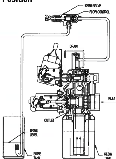
2 Brine Position
