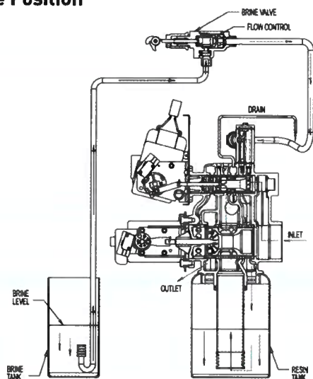
3 Brine Position
