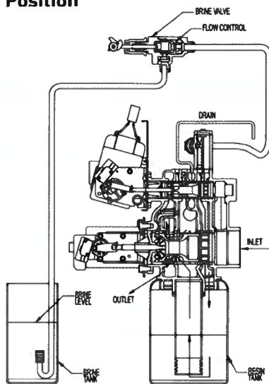
2 Backwash Position
